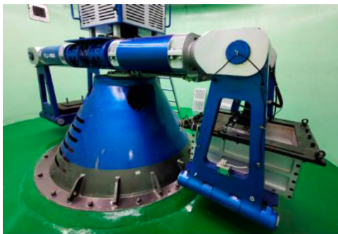
Figure 2. The TLJ-100A centrifuge. (This figure is available in colour online.)
